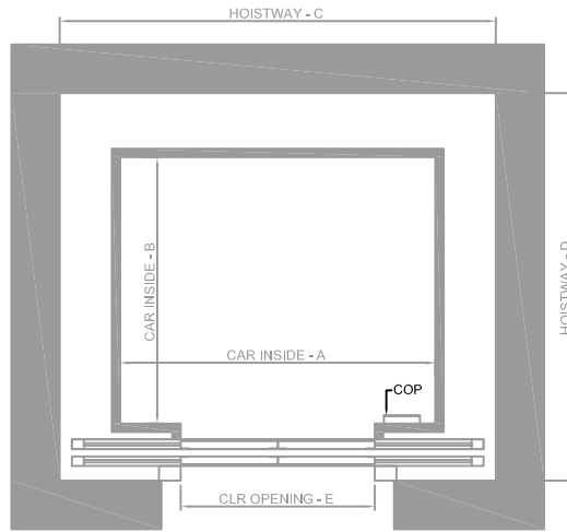
HOISTWAY PLAN
